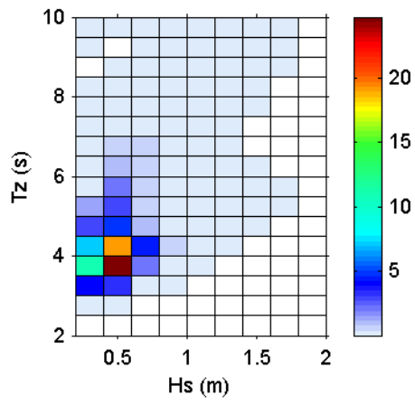
Swanage Pier 2007 to 2011 - Joint distribution (% of occurrence)
