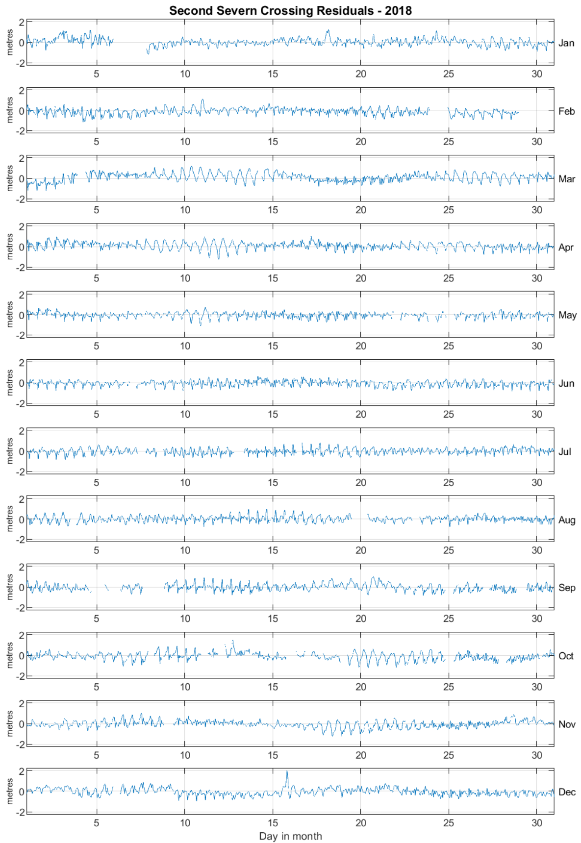
Figure 1: Severn Bridge residuals for 2018
